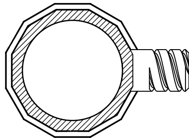
SECTION B-B SCALE 4.5 : 1
