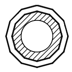
SECTION C-C SCALE 4.5 : 1
